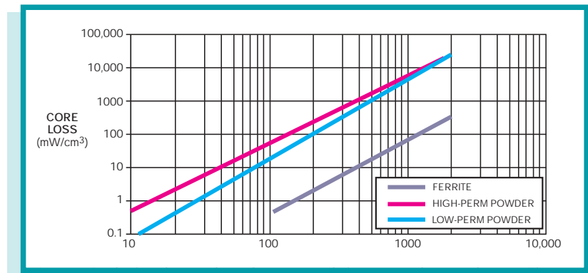
Figure 3. Reducing the number of turns greatly increases the core losses. The increased core loss and the variability of the inductance make the use of high-permeability powder cores impractical.
