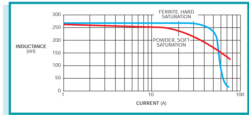
Figure 2. A distributed-gap powder core exhibits a soft-saturation characteristic.
