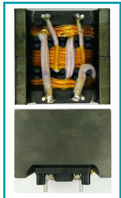
Fig. 9: Transformer prototype sample.
