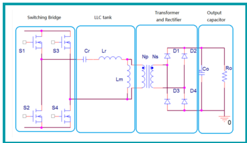
Fig. 1: LLC Converter
