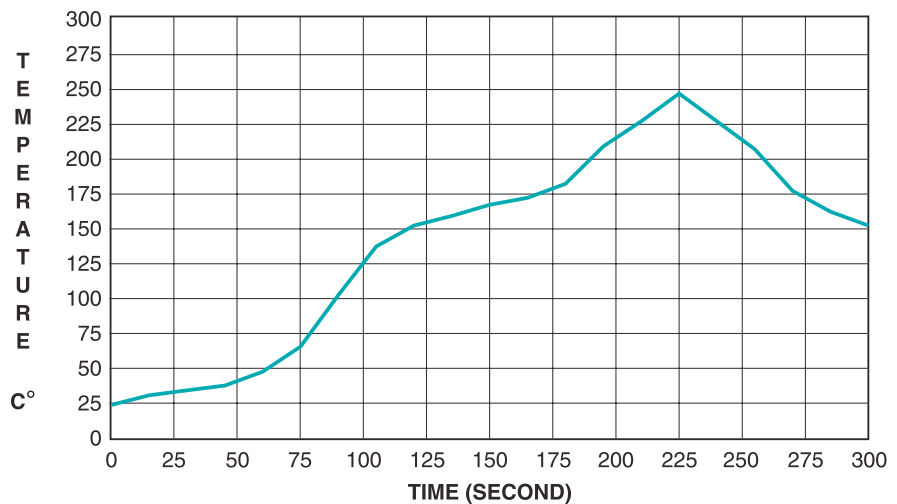
Recommended Solder Heat Resistance Profil
